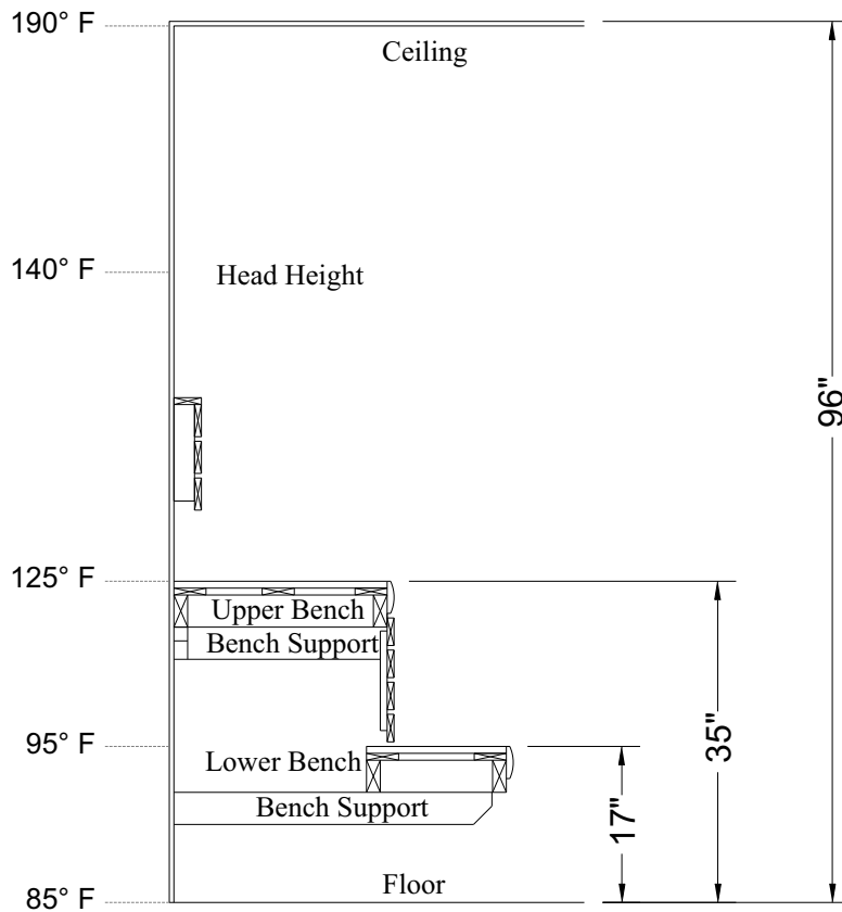
DIAGRAM 7: ROOM TEMPERATURES
