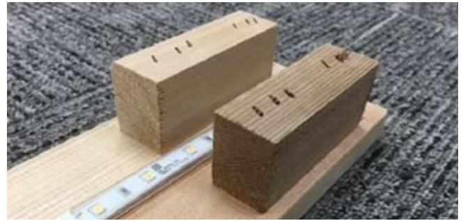
Backside view of a simple valance built from 1x4 cedar with 1x1 stand-off legs.
